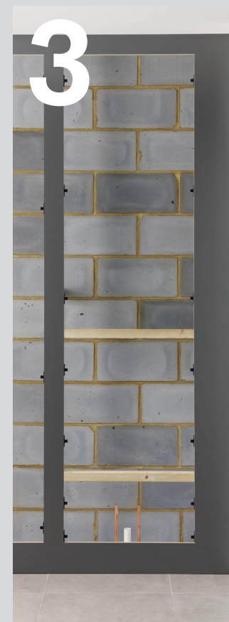
03 Attach fixing clips to the inside edge of the vertical flashgaps, repeat process on back face of panels.
